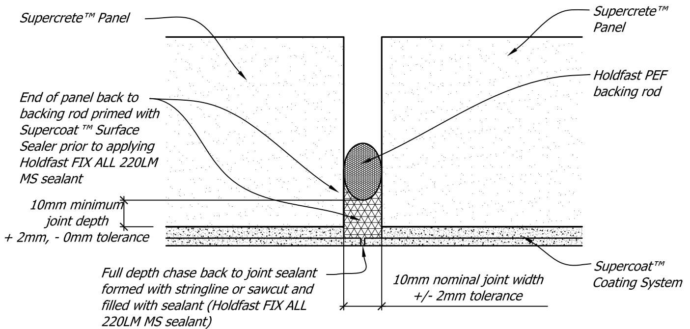
Vertical Control Joint Detail (Plan Section)
