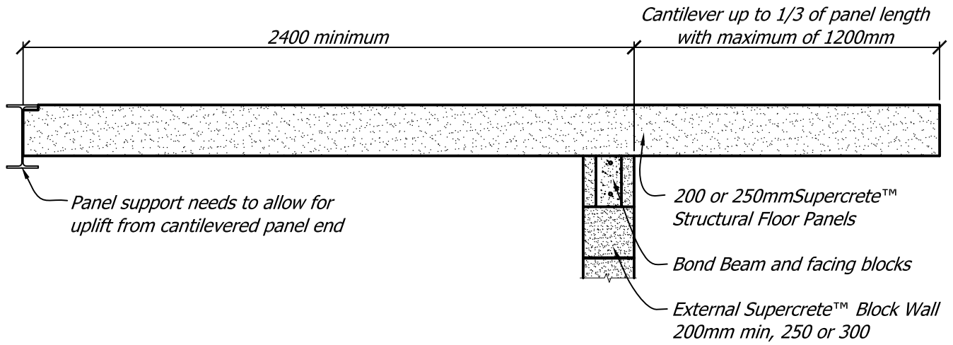
Cantilevered panel restraints for 200 & 250mm Supercrete™ Structural Floor Panels
