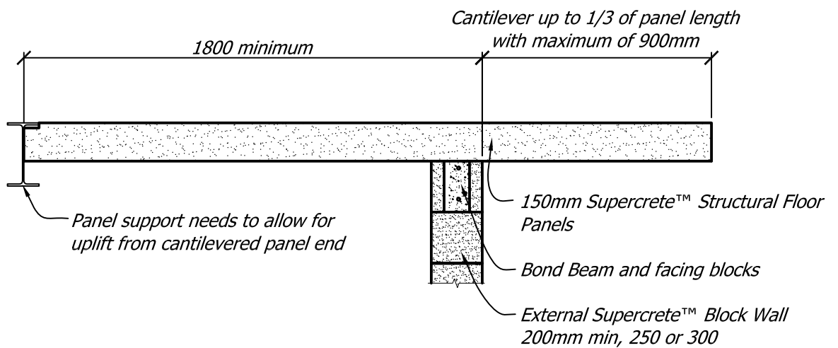
Cantilevered panel restraints for 150mm Supercrete™ Structural Floor Panels
