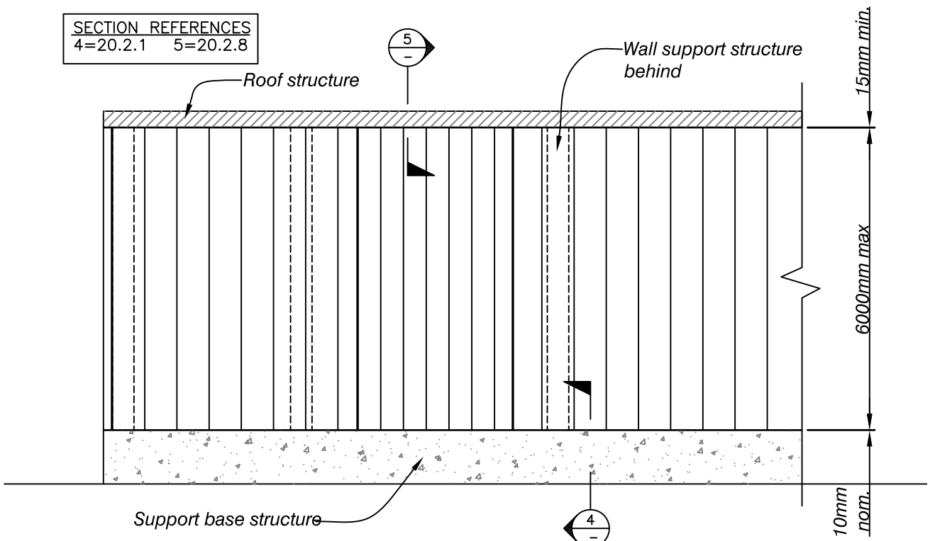
Elevation View - 1
